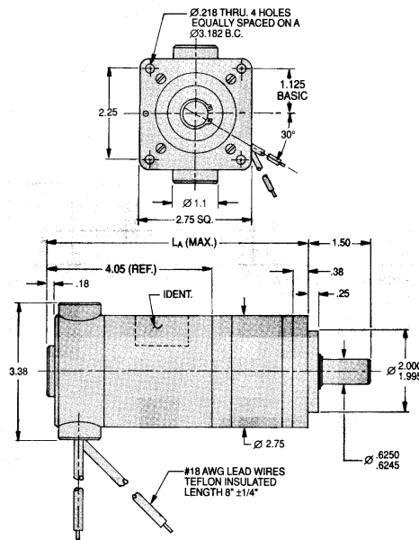
MODEL HIR GEARMOTOR
